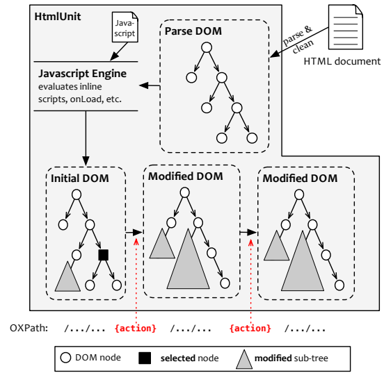
Figure 2: OXPath Event-Actions
